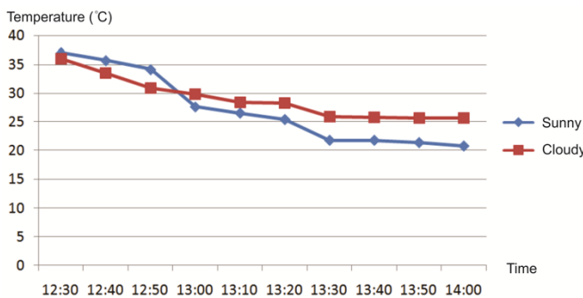
Figure 7. Cooling temperature with R22 type of 2 bars refrigerant pressure
