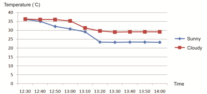
Figure 5. Cooling temperature with R134a type of 2 bars refrigerant pressure
