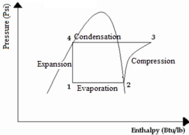
Figure 3. Ideal steam compression in Pressure-vs-enthalpy
