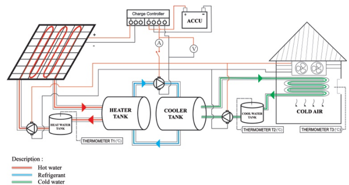
Figure 1. Schematic diagram of cooling system
